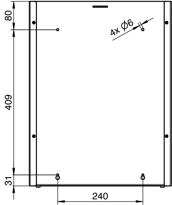
Bohrbild I drilling pattern
