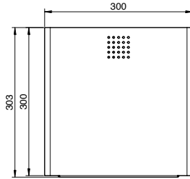
Bohrbild I drilling pattern
