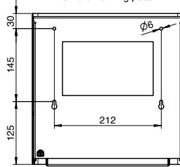
Bohrbild I drilling pattern
