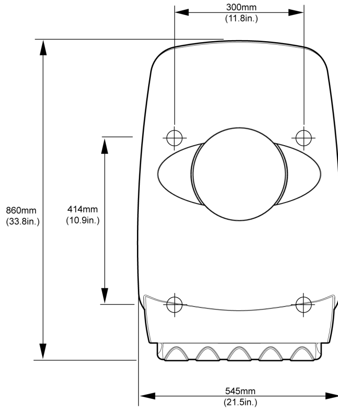
Vertical Baby Changing Unit Scale 1:10
